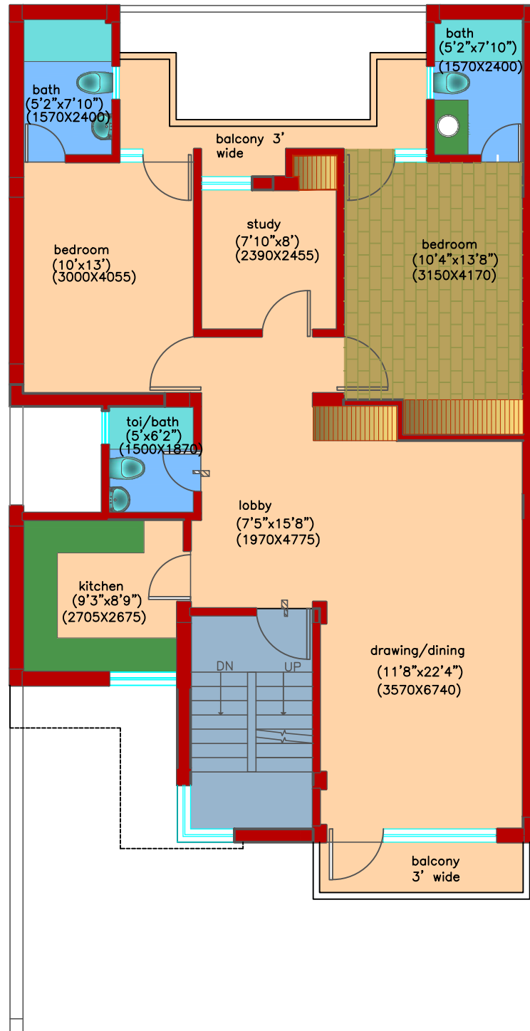
First Floor plan SUPER AREA=1310 SQ.FT.
