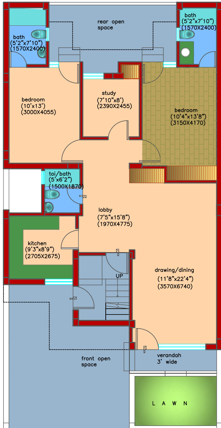
Ground Floor plan SUPER AREA=1270 SQ.FT.
