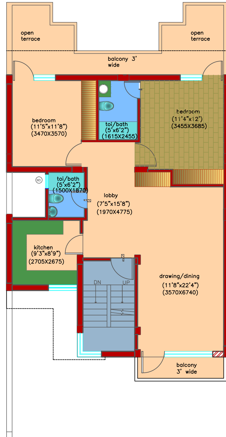
Second Floor plan SUPER AREA=1198 SQ.FT.
