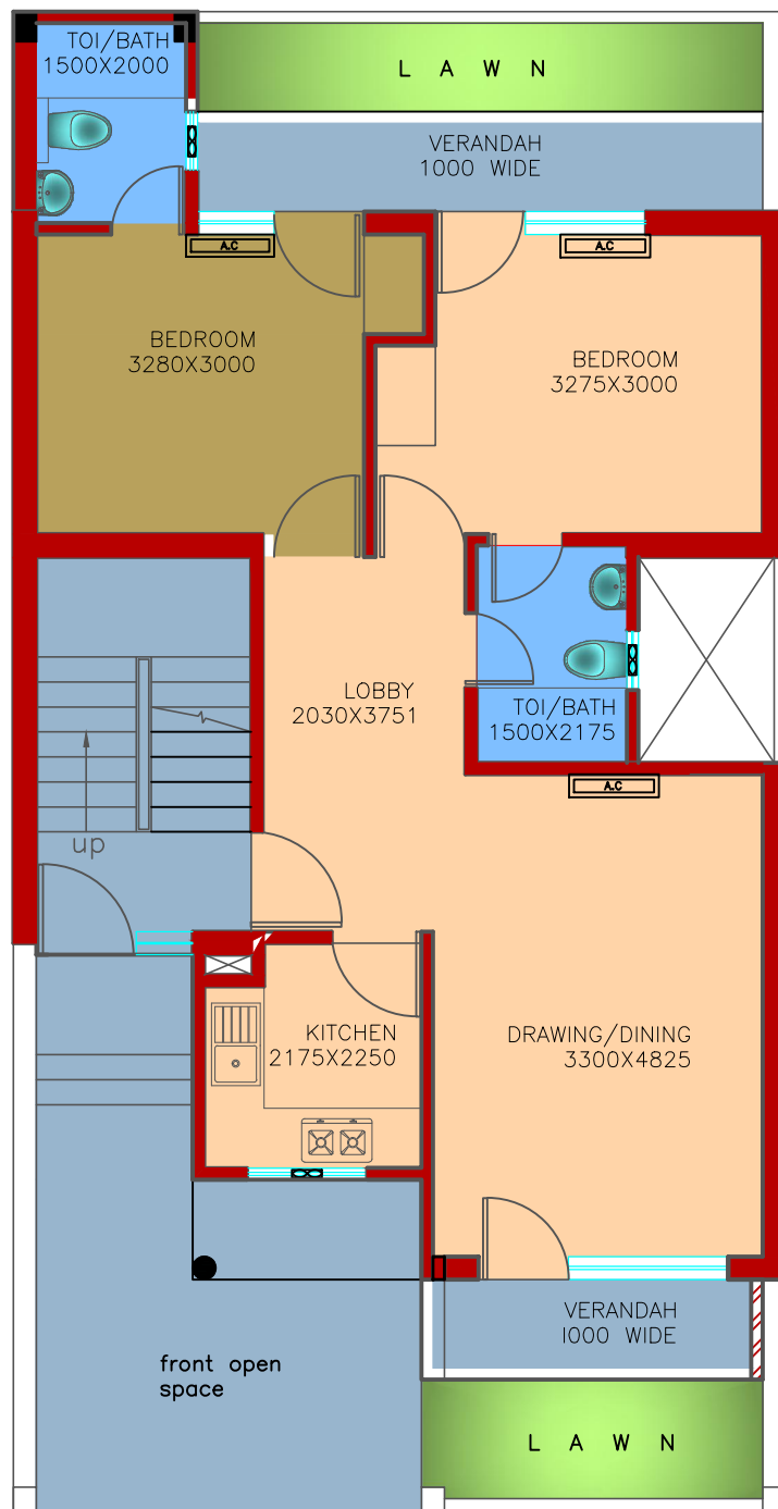
GROUND FLOOR PLAN SUPER AREA 940 SQ.FT.
